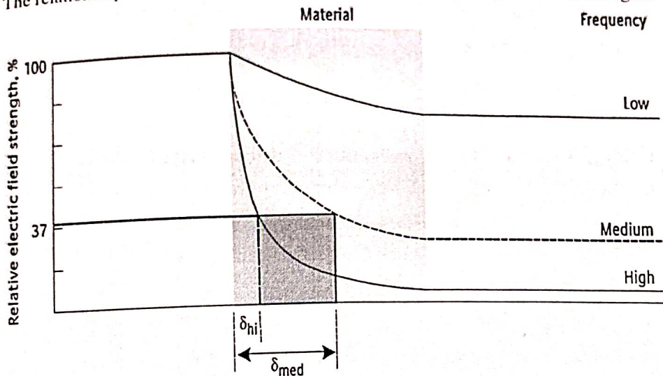
Figure 3. Relation between RF wave depth penetration and emitted frequency from generator (4).
