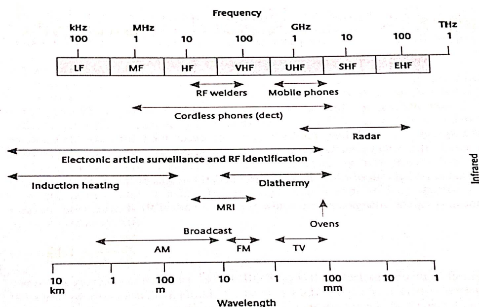
Figure 1. Electromagnetic fields according to the frequency ranges (4).
